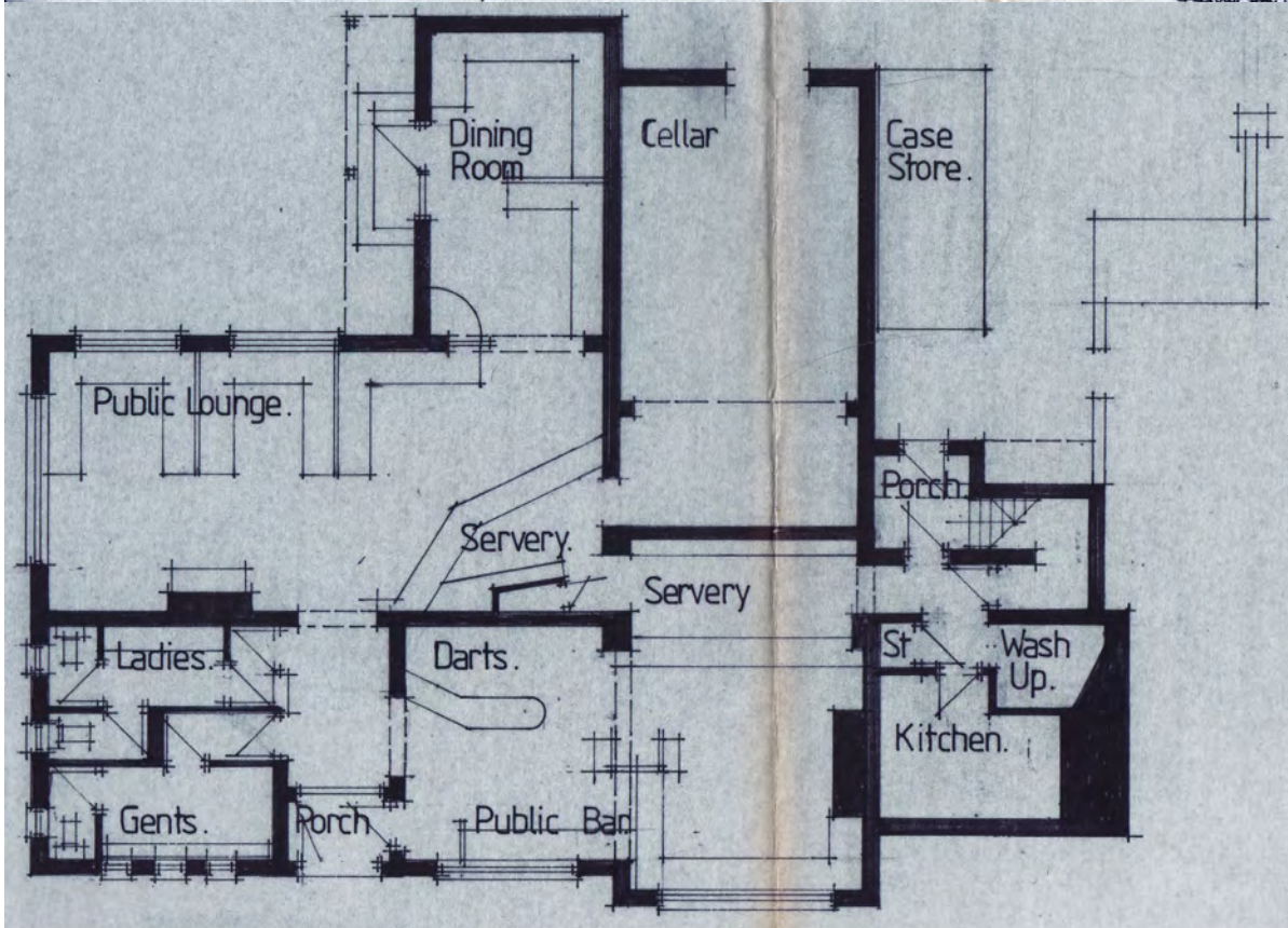
GROUND FLOOR PLAN as EXISTING. Scale: 1/100
